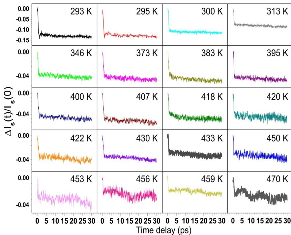
Supplementary Figure 1: Differential scattering from V_3O_5 as a function of temperature.
