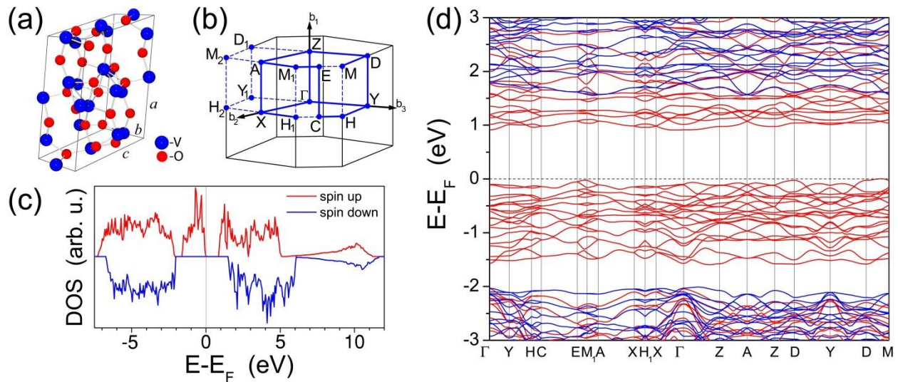
Supplementary Figure 2: (a) V_3O_5 unit cell. (b) Brillouin zones. (c) Density of states and (d) electronic energy bands of low-T V_3O_5 .
